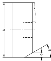
Position of the fastening screws for lathe chucks with cylindrical centring mount size 74-630
