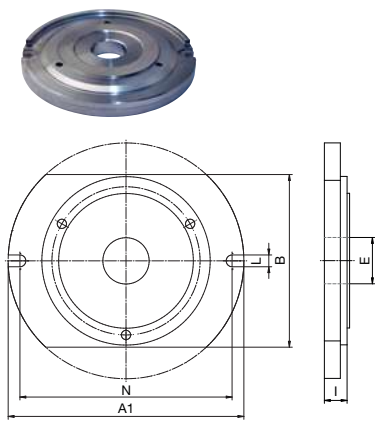
A09 Base plates for lathe chucks with cylindrical centre mount, DIN 6350
