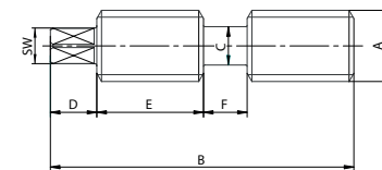
Adjusting spindle
