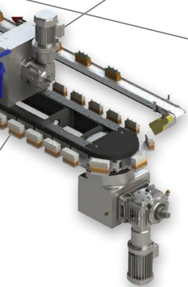
Camco LPP Linear Parts Handler with Robohand Grippers
